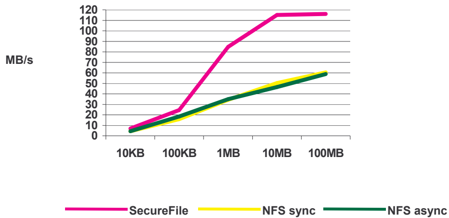
Insert/Write Performance
