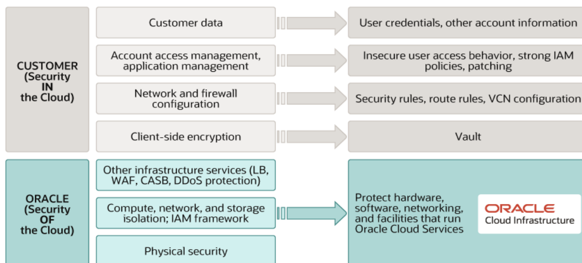
Figure 2: Shared Security Model
